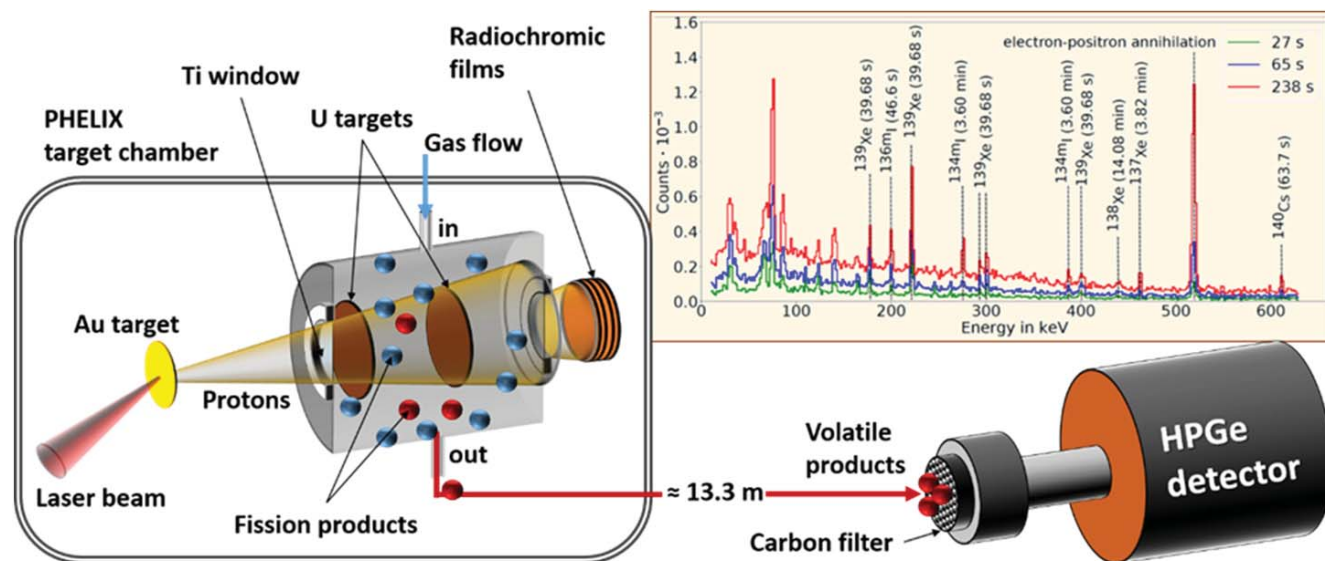
Schematic of the experimental setup and an obtained spectrum. Credit: Alexander Yakushev and Pascal Boller
