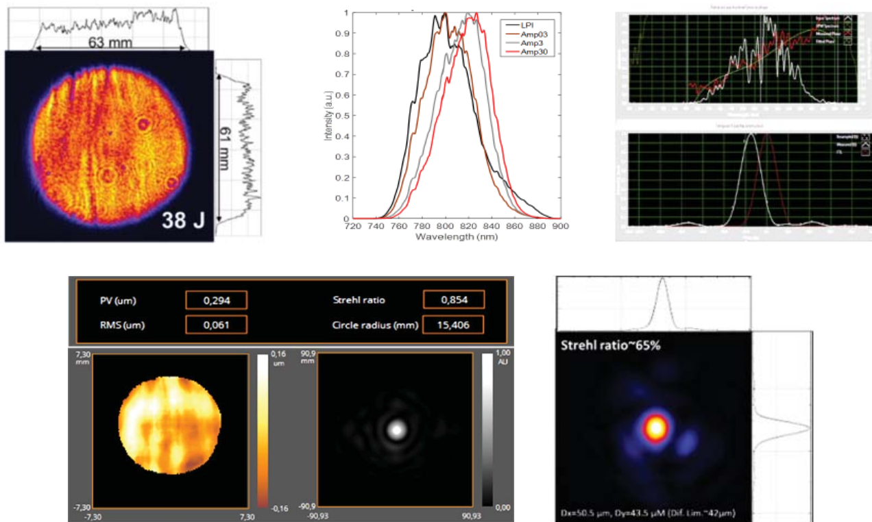
Fig. 1. Near-field beam profile at the output of the 4-th amplification stage (out of 5 in total) operating at 38 Joules (top row-left). Spectrum evolution throughout the laser chain: Front End (black line) to the 4-th Amplifier (red line) (top row-center). Wizzler measurement of the compressed pulses in the 1 PW beam line compressor (top row-right). Wavefront correction of the amplifiers output with 85% Strehl ratio (bottom row-left). Typical focal spot delivered on the target in the Long Focus Area (bottom row-right)
