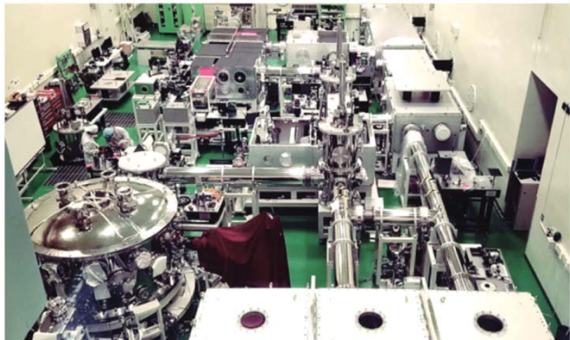
Experimental area for the 4-PW laser
