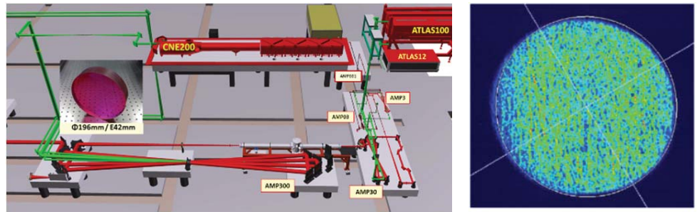
Fig. 2. Schematic of the complete amplification and pump section of the Apollon laser (left). Near field of the 200 Joules pump system already operational in our facility (right)
