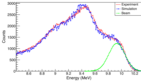
Fig. 3. In-beam energy measurement spectra for 9.9 MeV photons. The simulated data (blue) is superposed on the experimental data (red). The energy distribution of the beam (green) is added for comparison.
