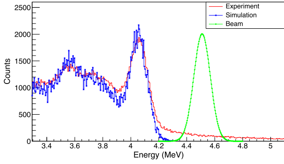
Fig. 5. The energy spectrum of Compton scattered 4.5 MeV photons. The simulated data (blue) is superposed on the experimental data (red). The energy distribution of the beam (green) is added for comparison.
