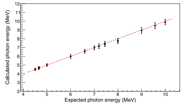
Fig. 4. The calculated versus expected incident photon energy for the 4.5 to 10 MeV range. The FWHM is shown as uncertainty for the calculated data. The dotted line (red) represents a guideline for equal values of calculated and expected incident photon energies.
