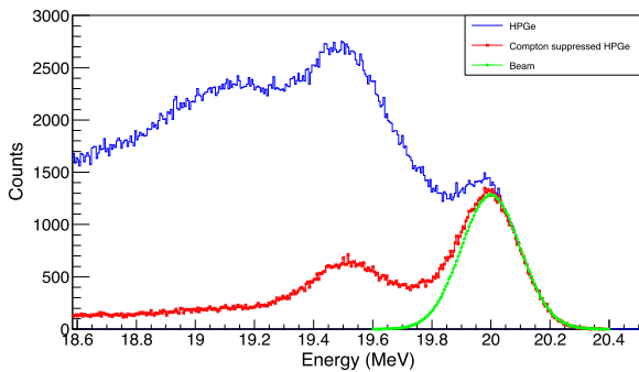
Fig. 9. Simulated in-beam spectra for an incident beam of 20 MeV. The blue line shows the results obtained using a simple germanium detector; the red line shows the results obtained for a Compton suppressed germanium detector.
