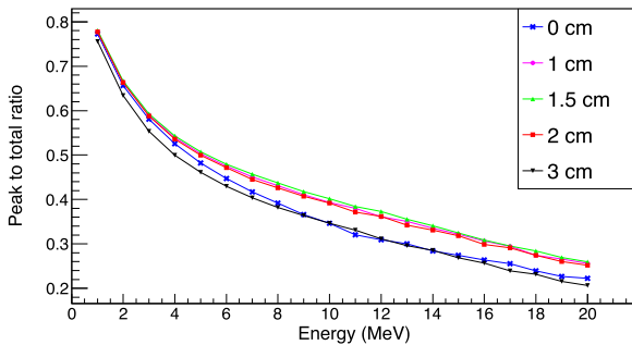
Fig. 10. P/T values obtained from simulated data using the proposed ELI-NP setup. The figure shows the results obtained for multiple positions of the beam with respect to the center of the detector.
