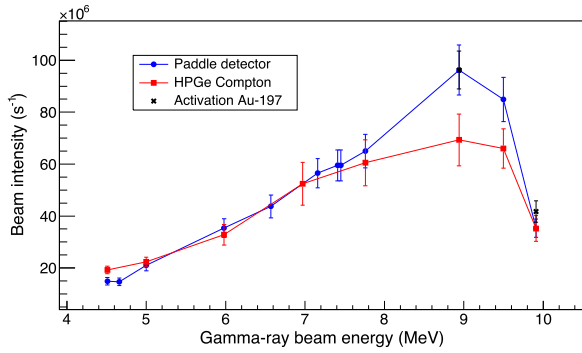
Fig. 6. Beam intensity results for the 4.5 to 10 MeV range using Compton scattering and the paddle detector. Absolute values were obtained by using ^{197}\text{Au} activation.
