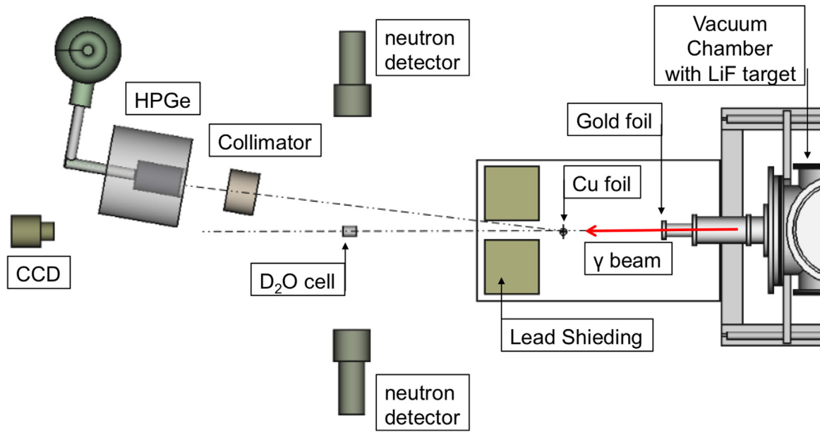
Fig. 1. The layout of the experimental arrangement in the Upstream Target Room (drawing not to scale). The vacuum chamber housed a LiF target and a silicon detector array for detecting charged particles from the photodisintegration of ^7\text{Li} . The other items in the setup were used for the characterization of the \gamma -ray beam.
