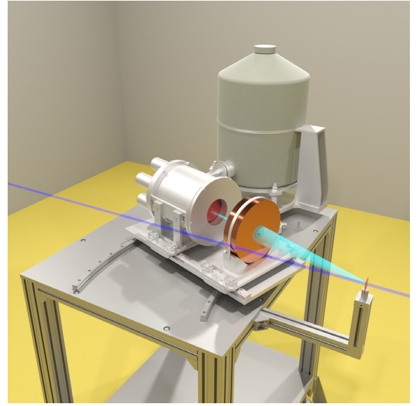
Fig. 7. Proposed setup for energy and intensity measurements at ELI-NP.
