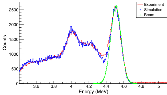
Fig. 2. In-beam energy measurement spectra for 4.5 MeV photons. The simulated data (blue) is superposed on the experimental data (red). The energy distribution of the beam (green) is added for comparison.
